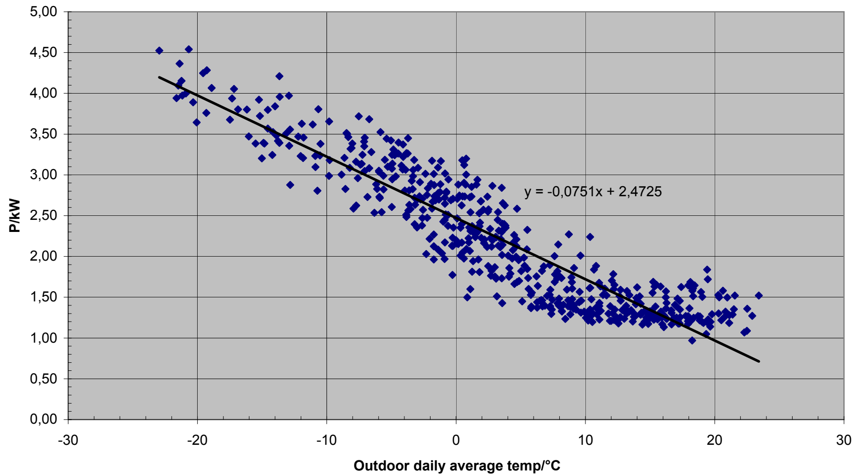
Average power versus outdoor temp average
