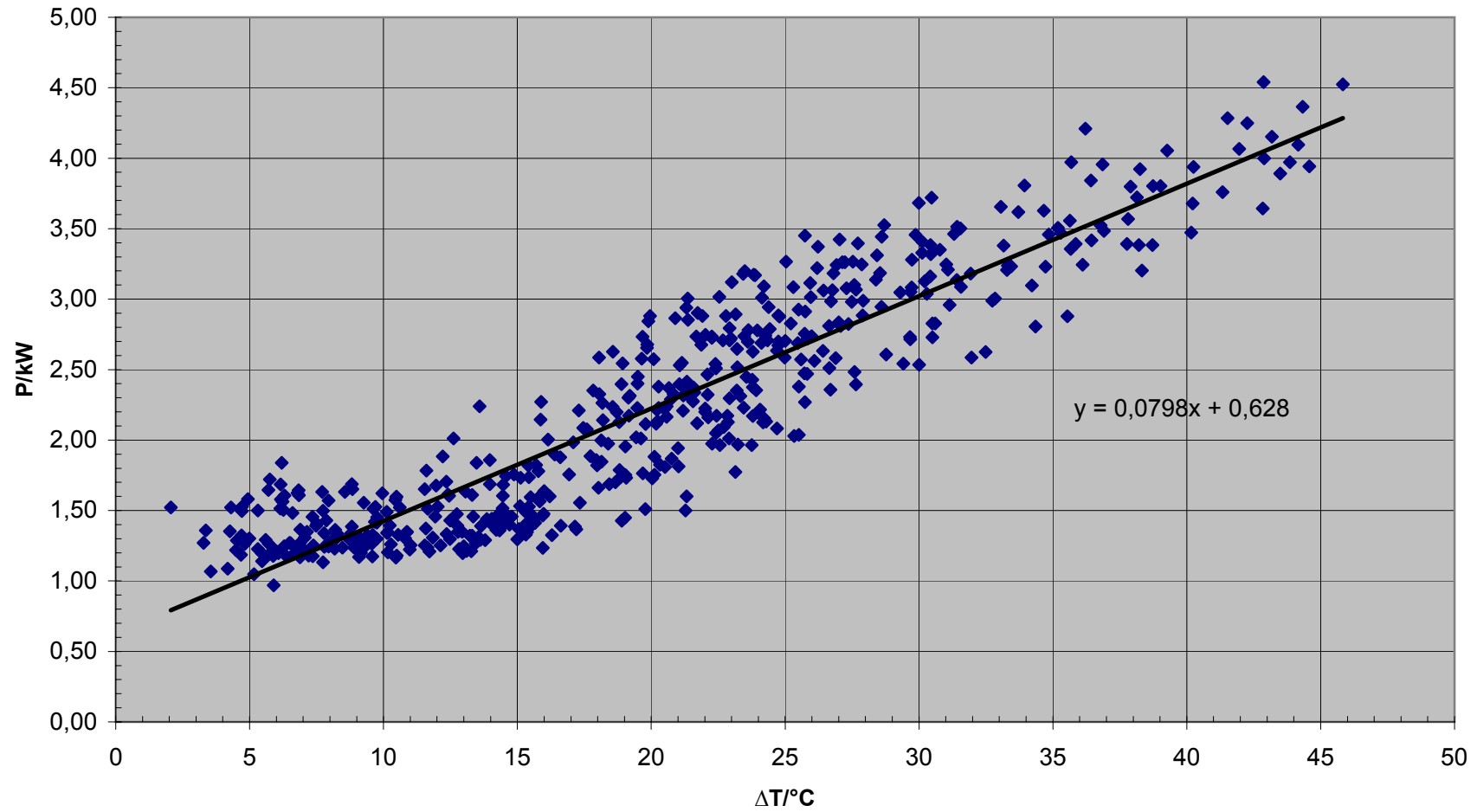
Average power versus \Delta T inside-outside
